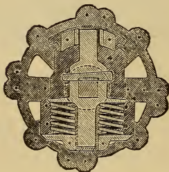
FIG. 43.—SECTION OF HUB.
